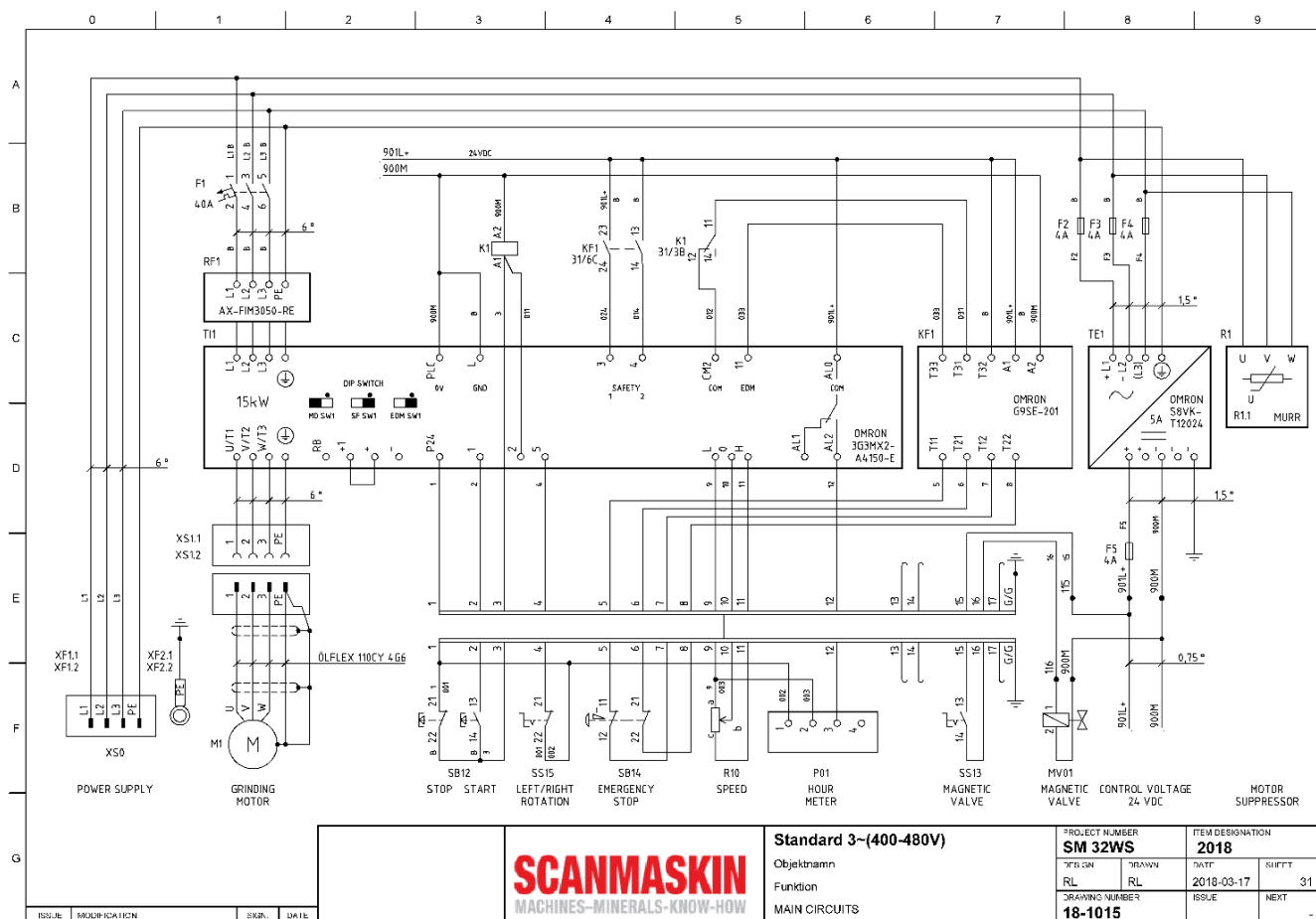
Figur 74 Kopplingsschema Scanmaskin 28 WS "Standard"
